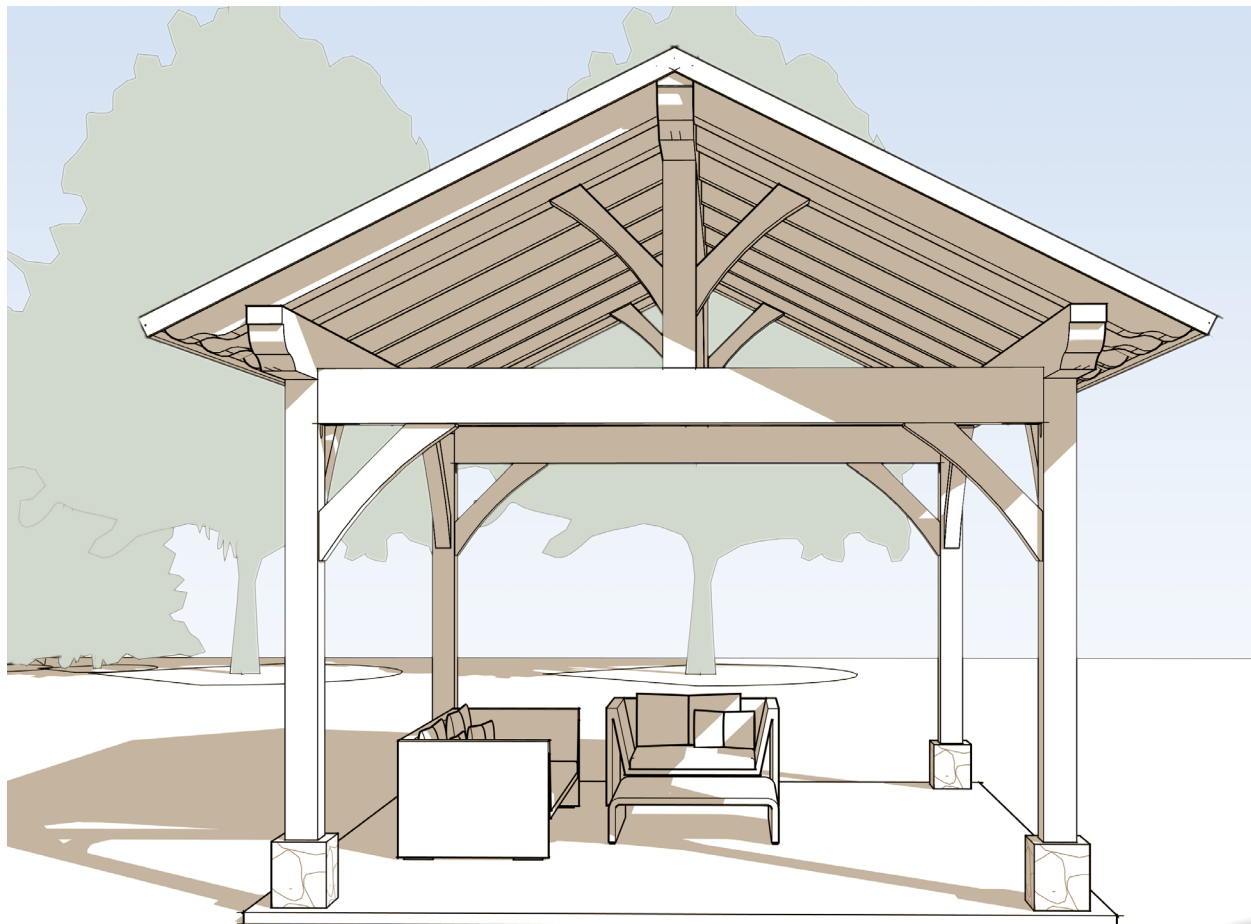
14' X 12' GAZEBO
