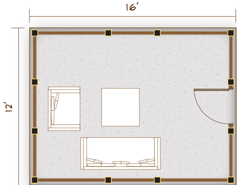
12' X 16' GAZEBO WITH SCREEN HOUSE OPTION
