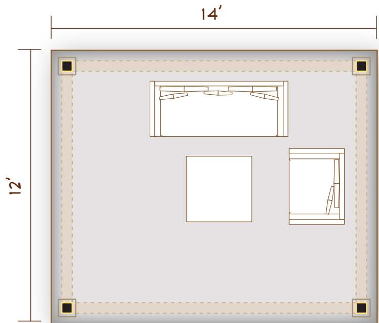
14' X 12' GAZEBO
